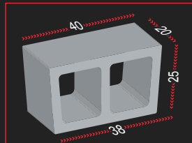
Hourdy 40x20x25x38 cm
